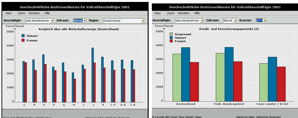
Figure 1: Dynamic presentation of results from the German SES 2001
